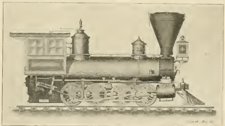
PERKINS EIGHT-WHEEL ENGINE.
